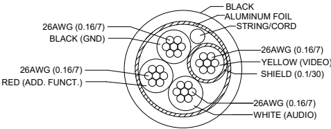
CABLE BUILDUP
