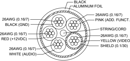
CABLE BUILDUP
